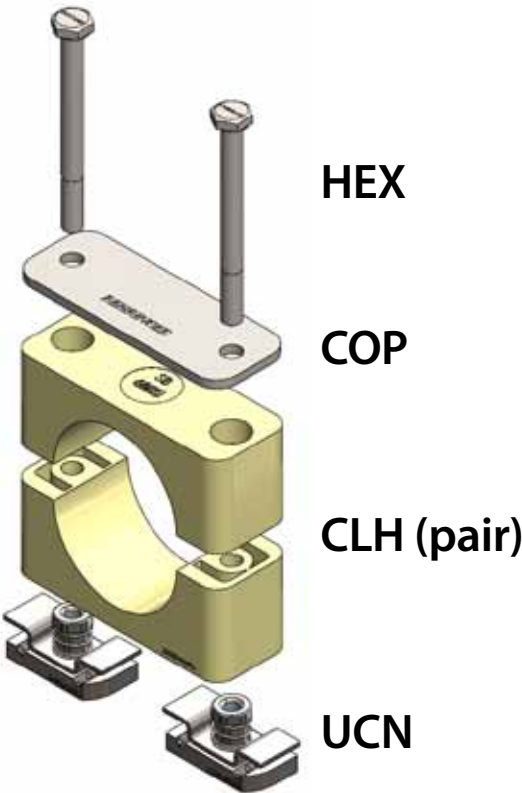
Figure 211 Unistrut Mount
