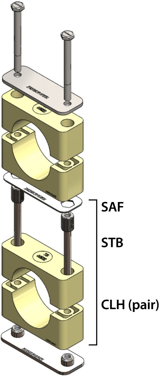
Figure 204 Stacking Kit
